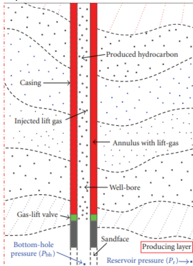
Figure 1. Schematic diagram of gas lift well.
