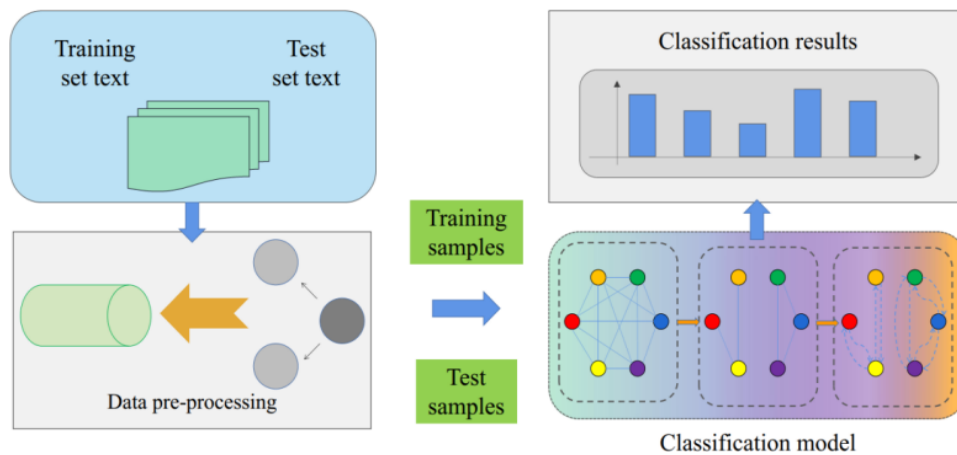
Figure 2. Model structure.
