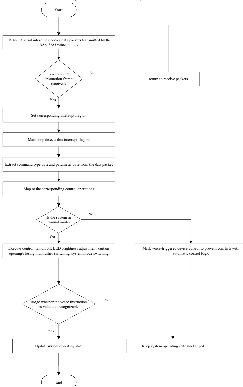
Figure 4. Flowchart of offline voice command parsing program.
