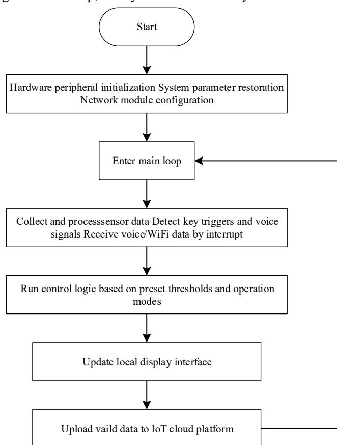
Figure 2. Overall system flow chart.
