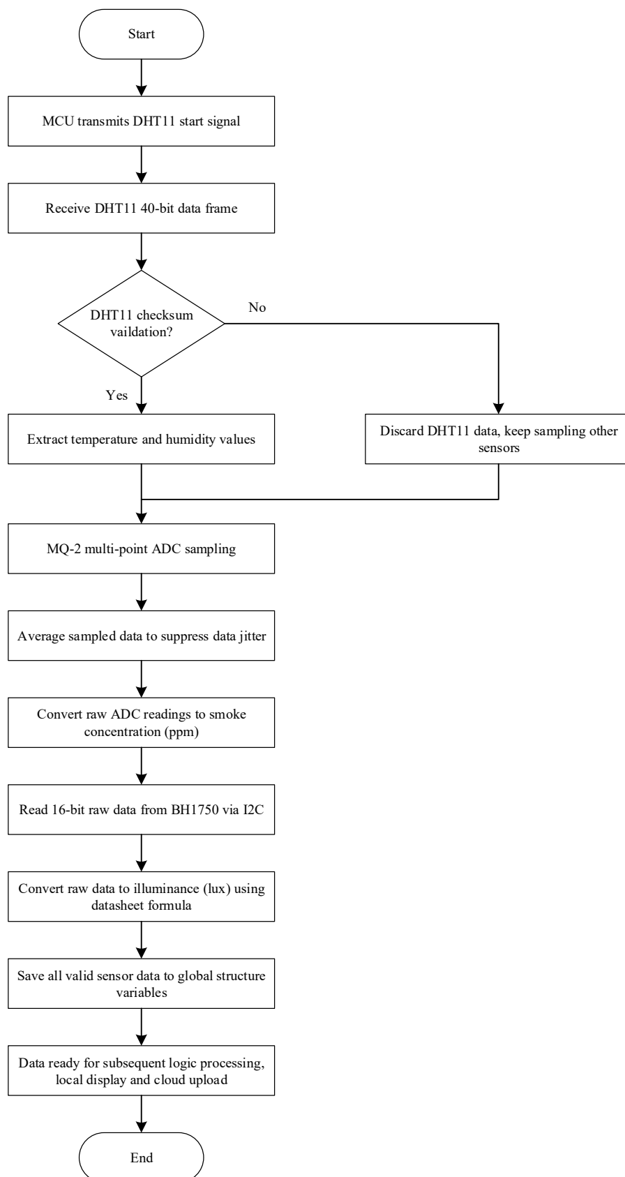
Figure 3. Flowchart of Multi-sensor Data Acquisition Program
