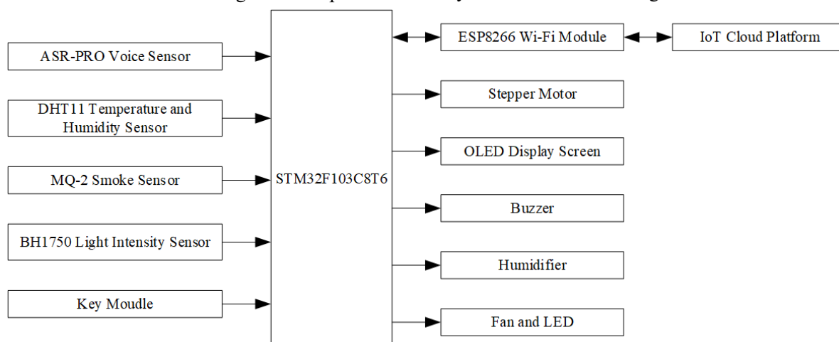
Figure 1. Overall system functional block diagram.
